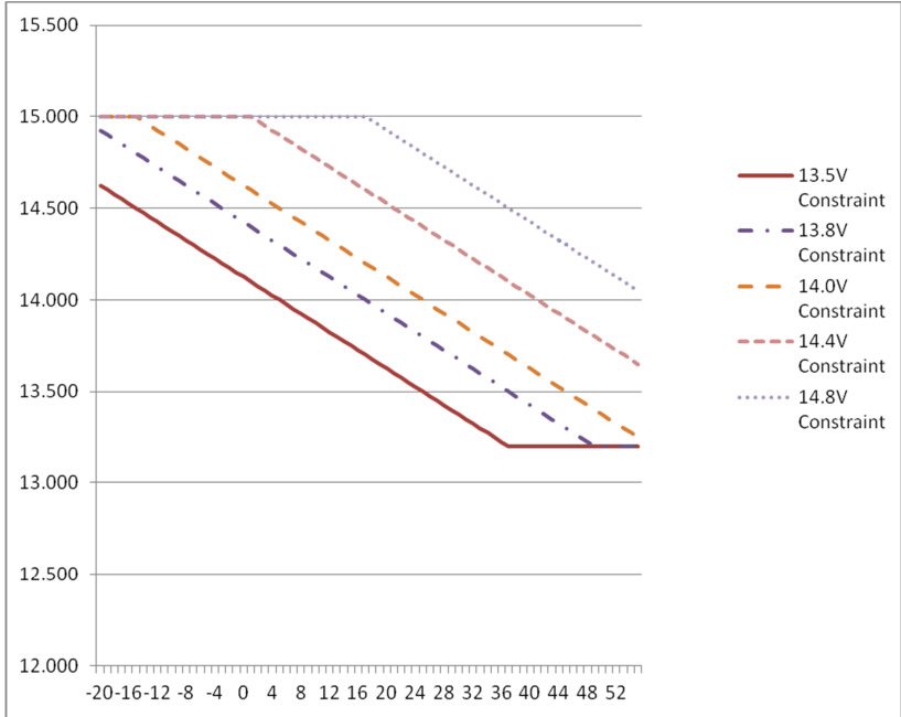
Figure 19 Temperature Compensation for 12V Model
