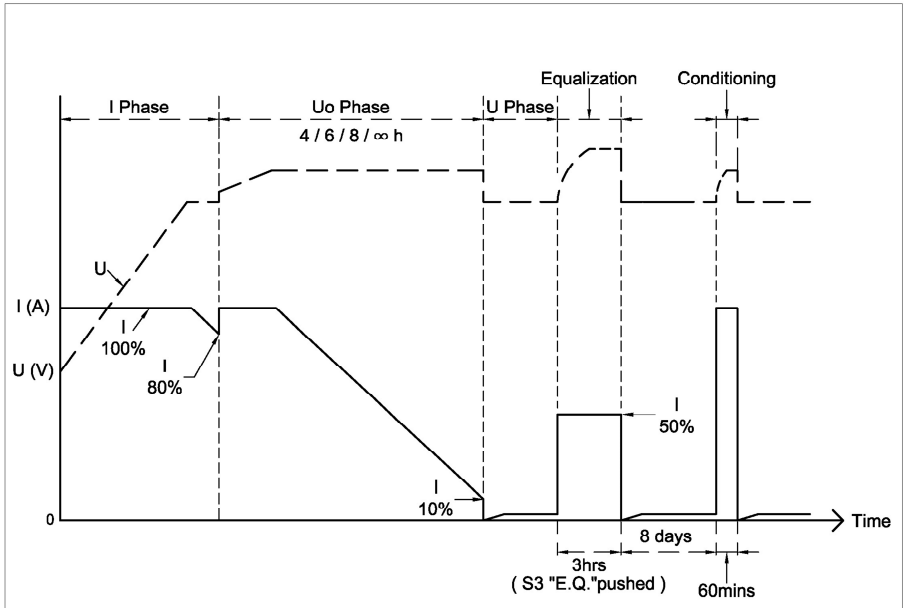
Figure 18 Charging characteristic
