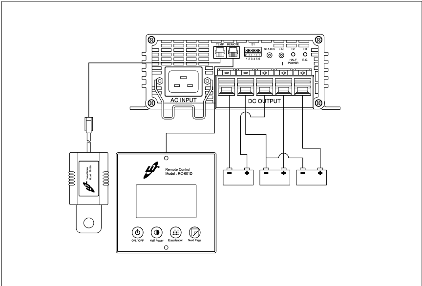
Figure 14 Making Connections (RC-601D)
