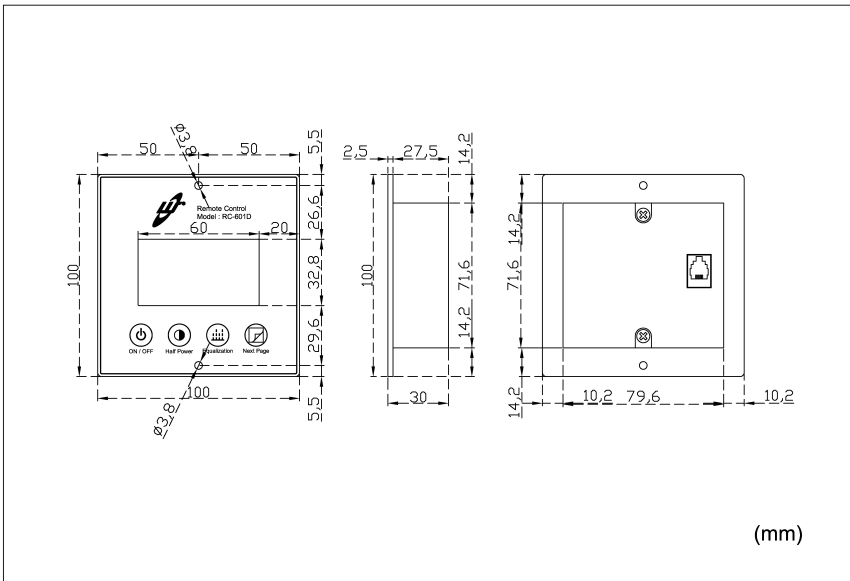
Figure 10 Remote Controller RC-601D Views
