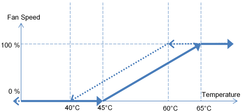
Figure 21 Fan Speed
