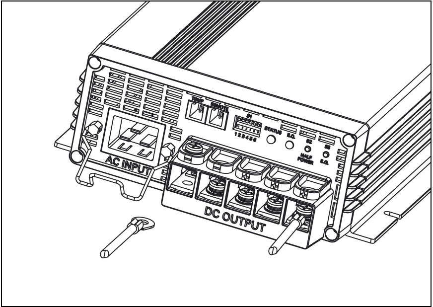
Figure 15 Cable Setup
