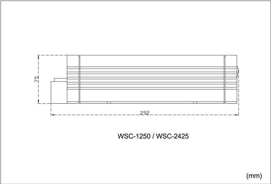
Figure 5 Charger Side View
