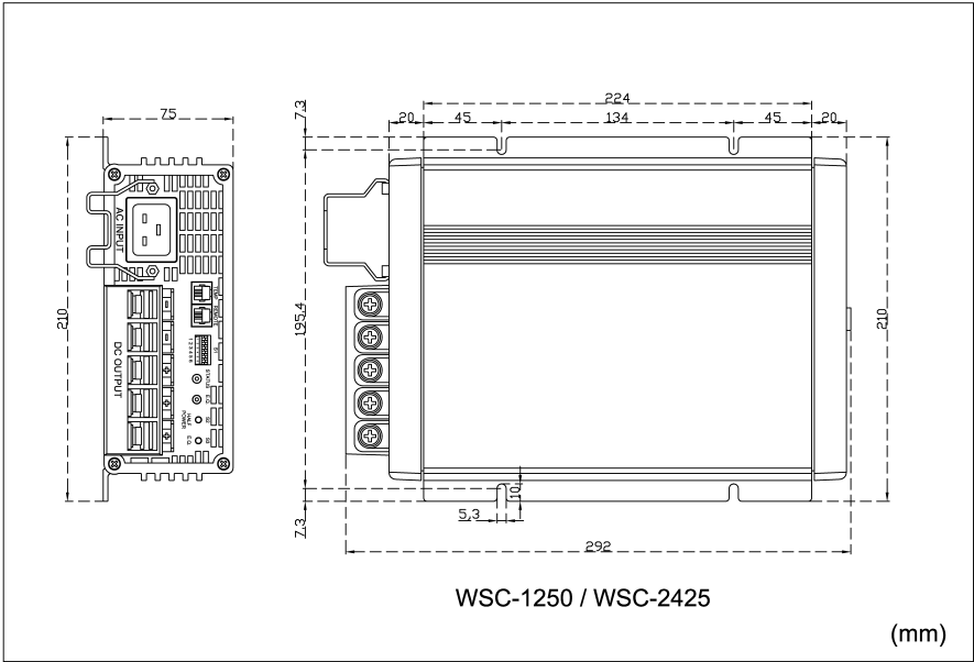
Figure 3 Charger Top View
