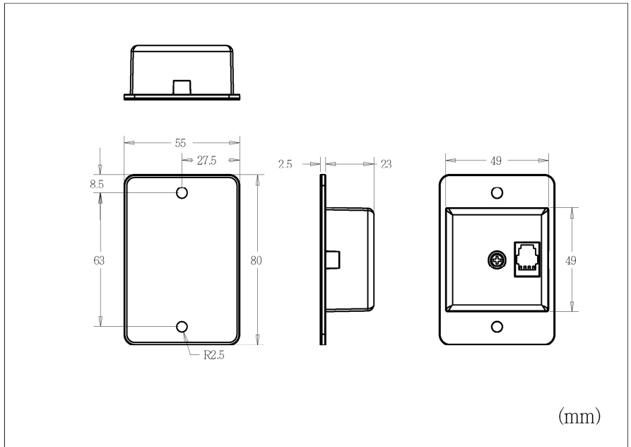
Figure 8 Remote Controller RC-600 Views
