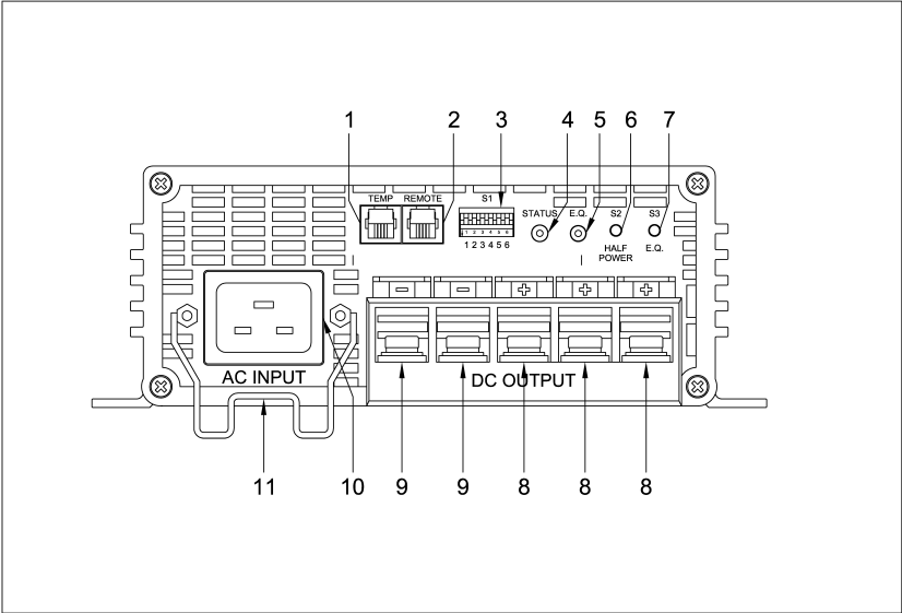
Figure 1 Charger Front View
