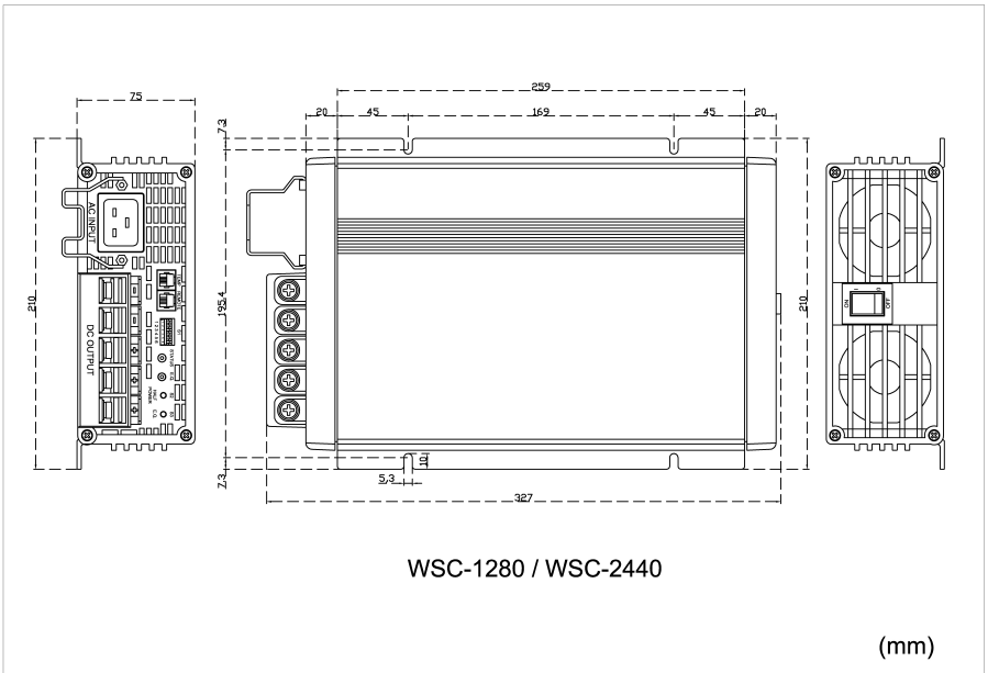
Figure 4 Charger Top View
