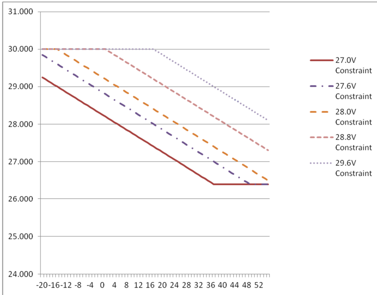
Figure 20 Temperature Compensation for 24V Model
