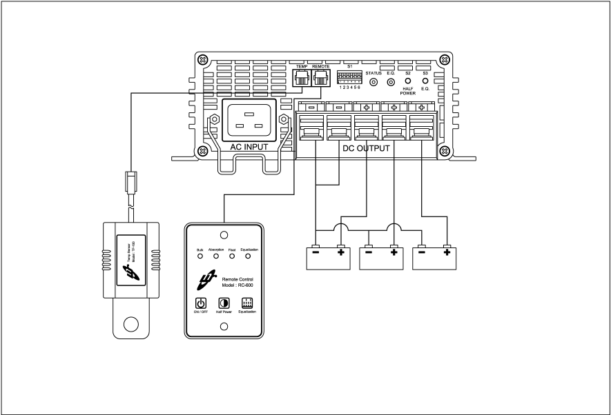
Figure 13 Making Connections (RC-600)
